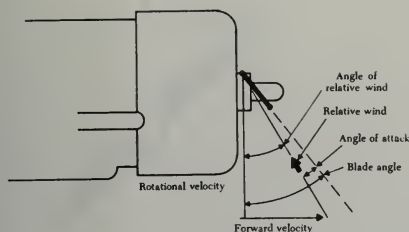
FIGURE 7-4. Propeller aerodynamic factors.
